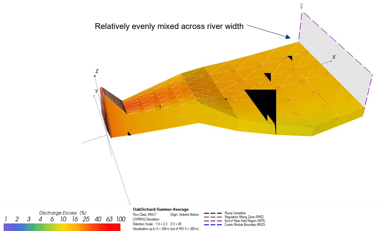
Figure 5.6 Effluent Plume Calculated for CORMIX for the Shallow Depth and Horizontal Discharge Scenarios
