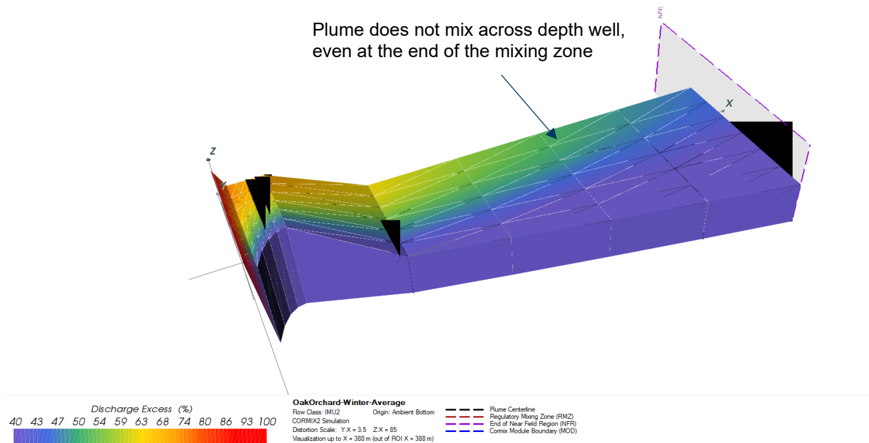
Figure 5.2 Effluent Plume Calculated for CORMIX for the Shallow Depth and Horizontal Discharge Scenarios
