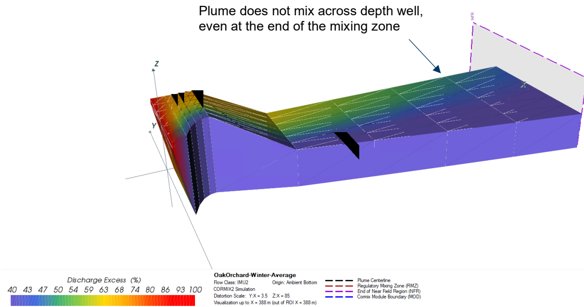
Figure 5.4 Effluent Plume Calculated for CORMIX for the Shallow Depth and Vertical Discharge Scenarios
