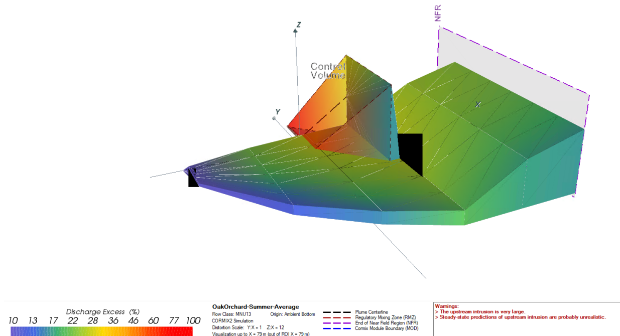
Figure 5.3 Effluent Plume Calculated for CORMIX for the Deep Depth and Vertical Discharge Scenarios, Showing Large Upstream Intrusion
