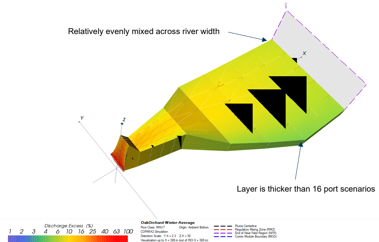
Figure 5.5 Effluent Plume Calculated for CORMIX for the Deep Depth and Horizontal Discharge Scenarios
