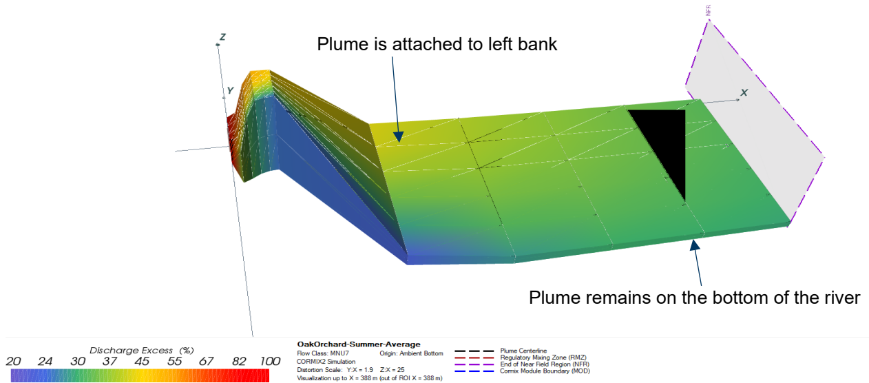
Figure 5.1 Effluent Plume Calculated for CORMIX for the Deep Depth and Horizontal Discharge Scenarios
